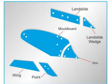
The Plough Body Construction
